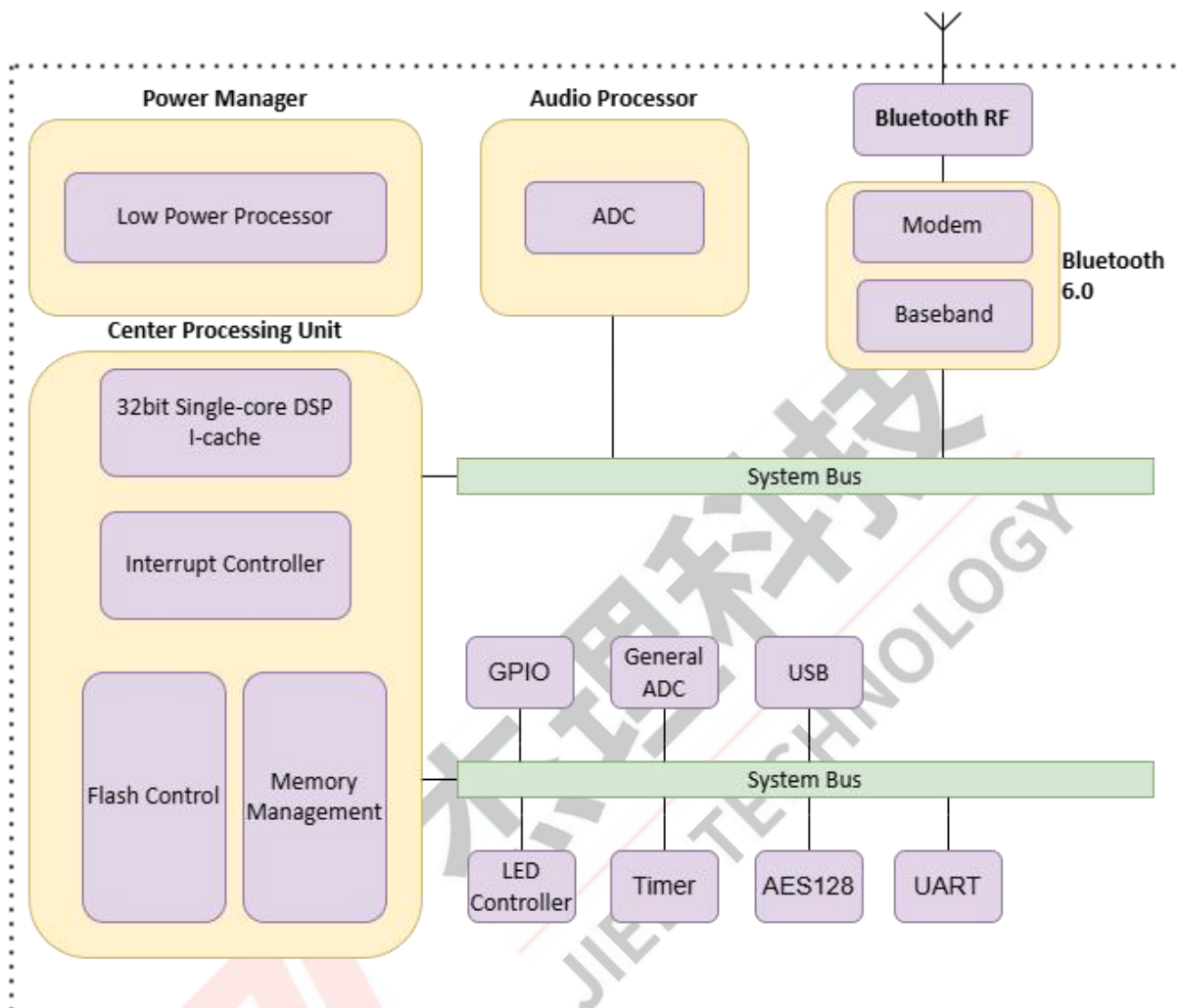
Figure 1-1 AW328A Block Diagram
