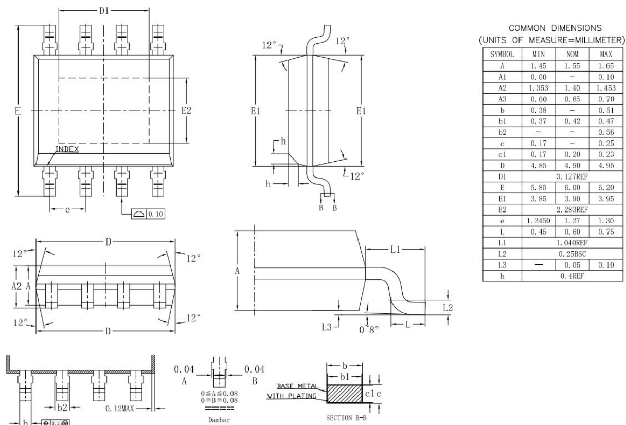
Figure 4-1 AW328A Package
