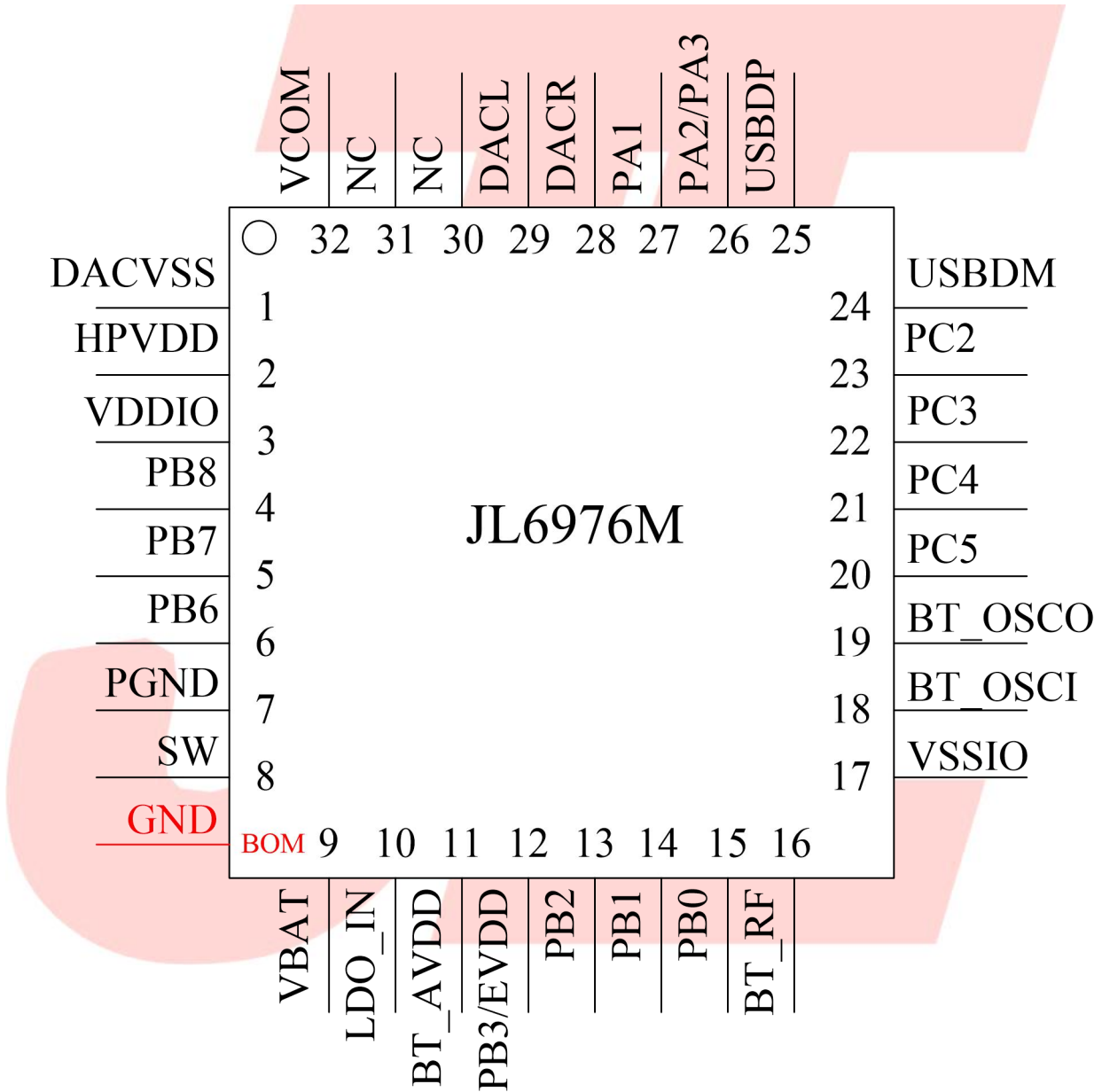
Figure 1-1 JL6976M Package Diagram
