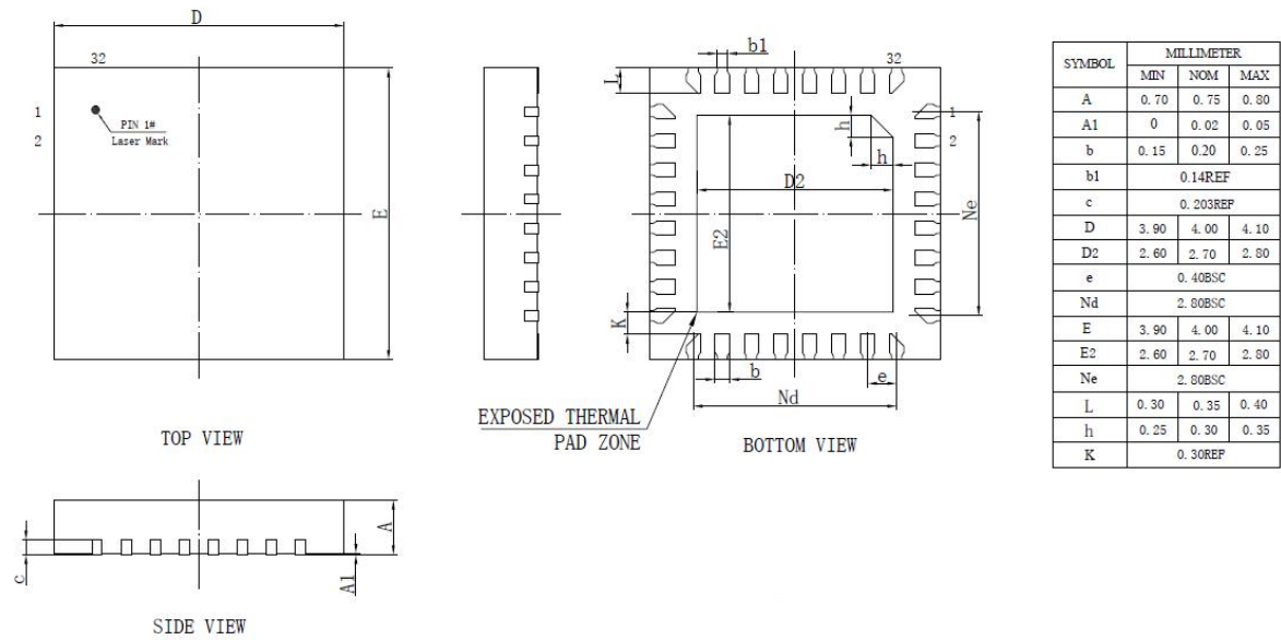
Figure 3-1 JL6976M Package
