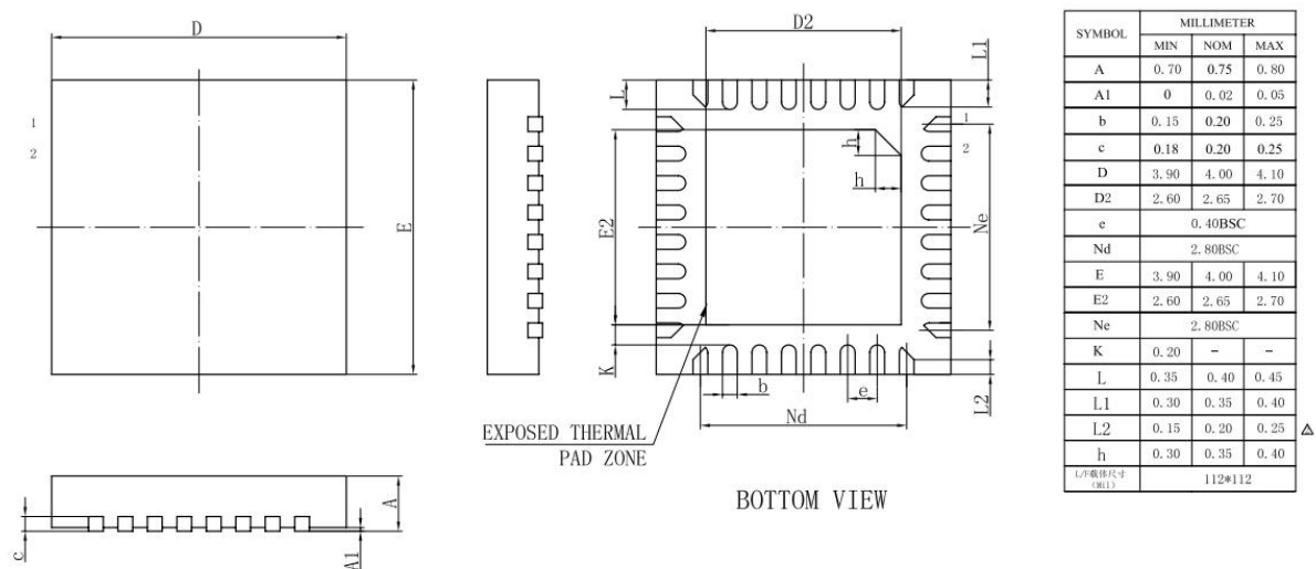
Figure 3-1 JL7006F Package
