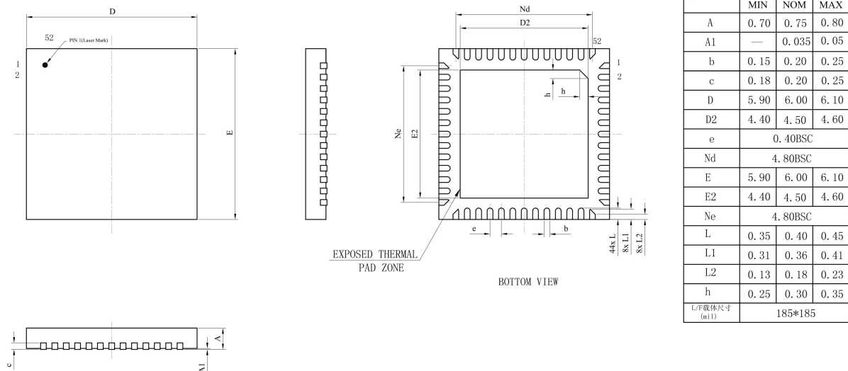
Figure 4-1 JL7012R Package
