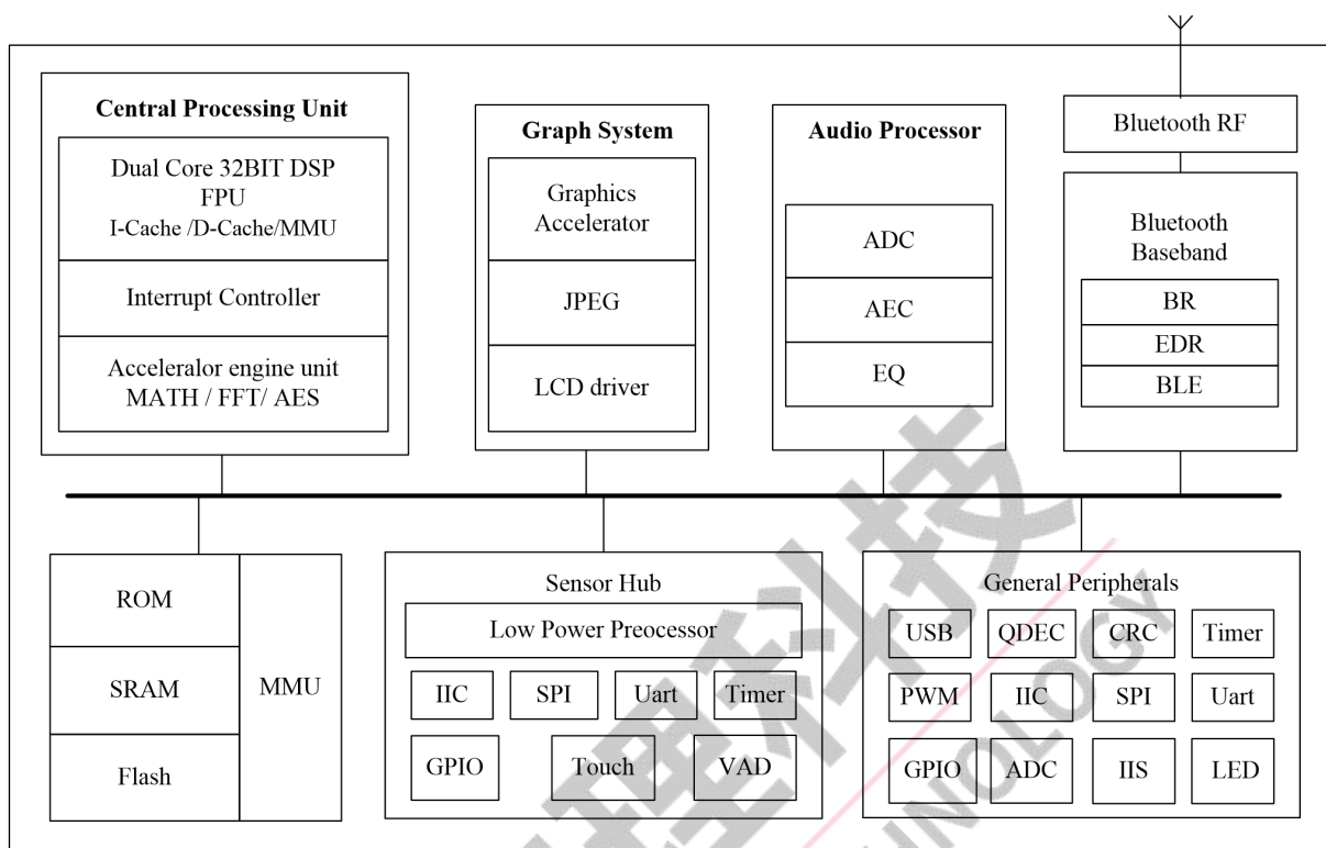
Figure 1-1 JL7012R Block Diagram
