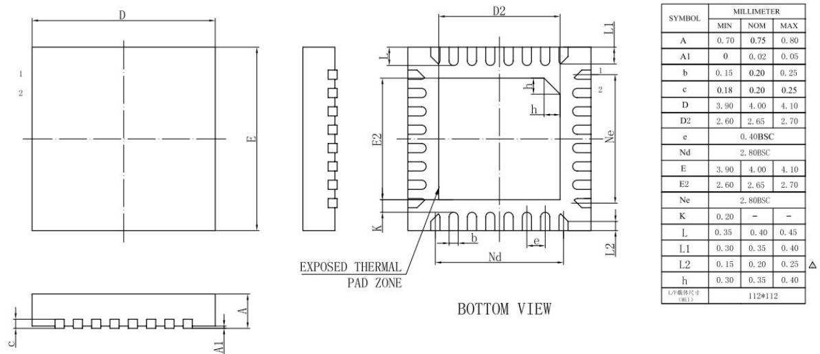
Figure 4-1 JL7016G Package
