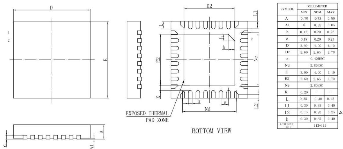
Figure 4-1 JL7016M Package
