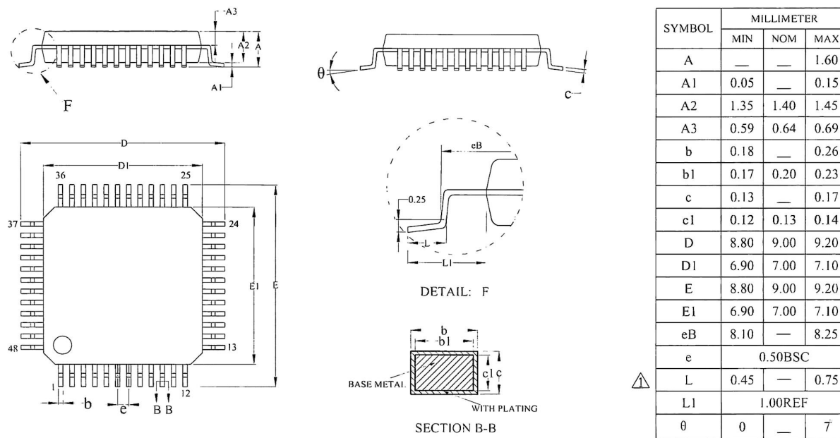
Figure 4-1 JL7031C Package
