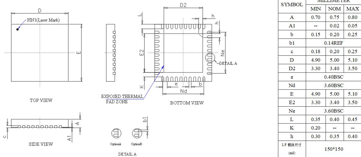
Figure 4-1 JL7032F Package
