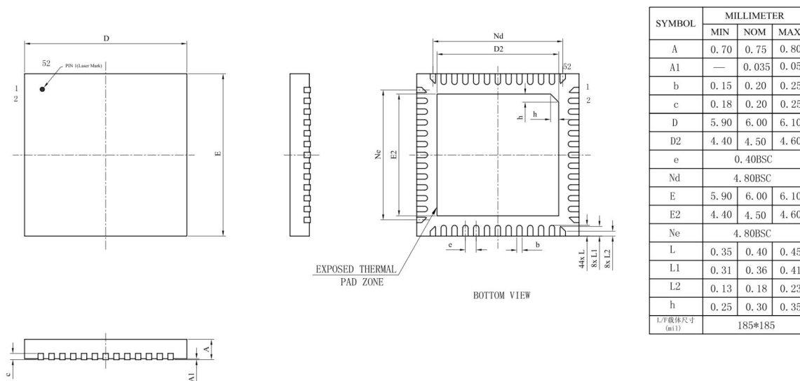
Figure 4-1 JL7034A Package
