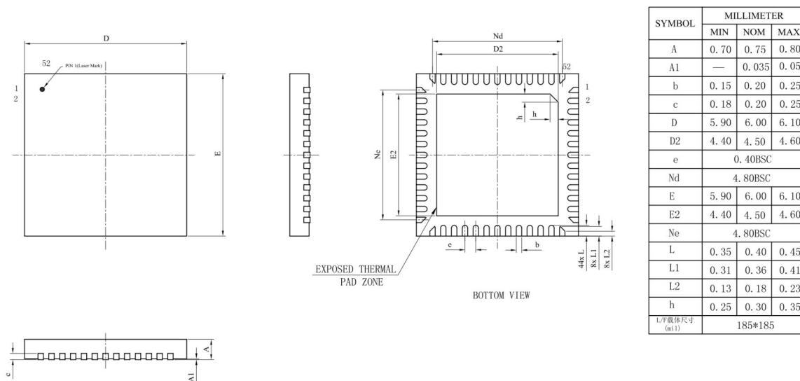
Figure 4-1 JL7034C Package
