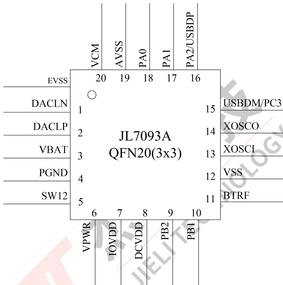
Figure 2-1 JL7093A Pin Assignment
