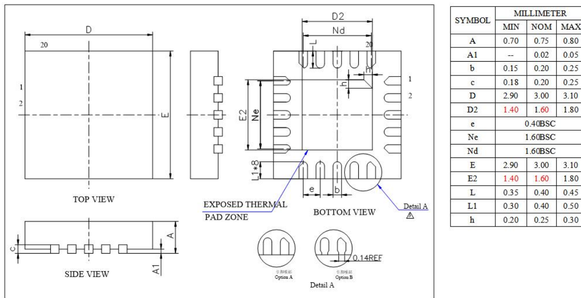
Figure 4-1 JL7093A Package
