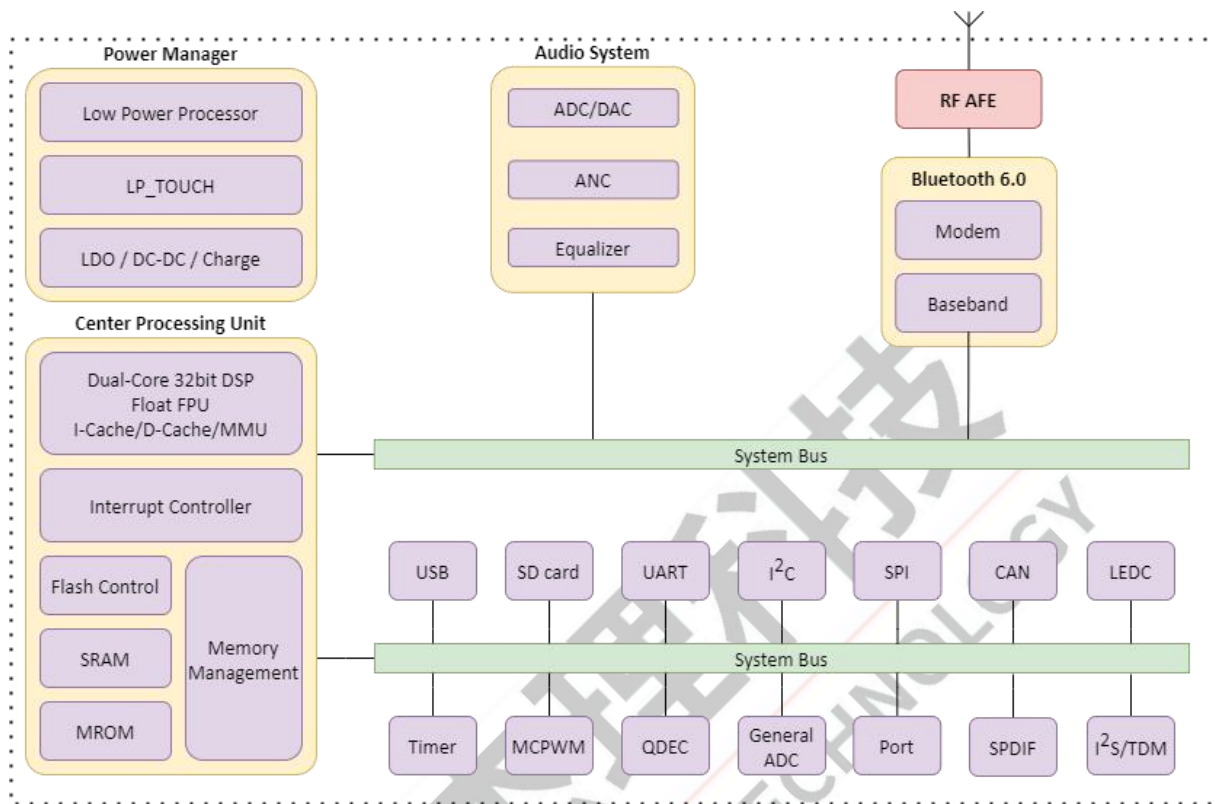
Figure 1-1 JL7093A Block Diagram
