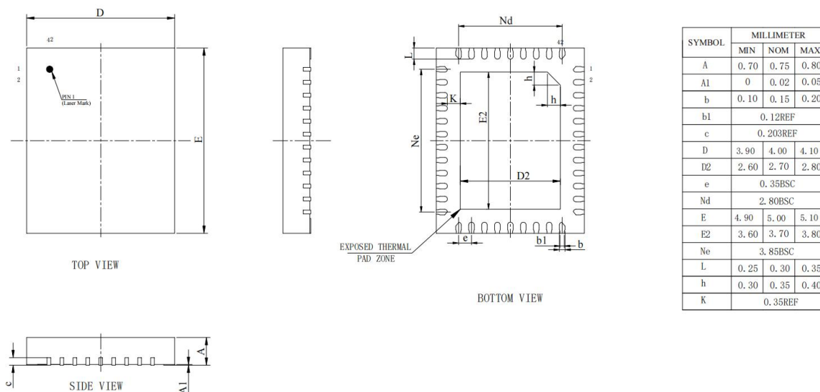
Figure 4-1 JL7094F Package
