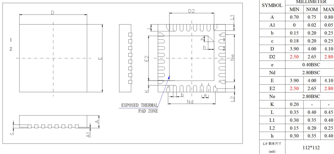
Figure 4-1 JL7096D Package
