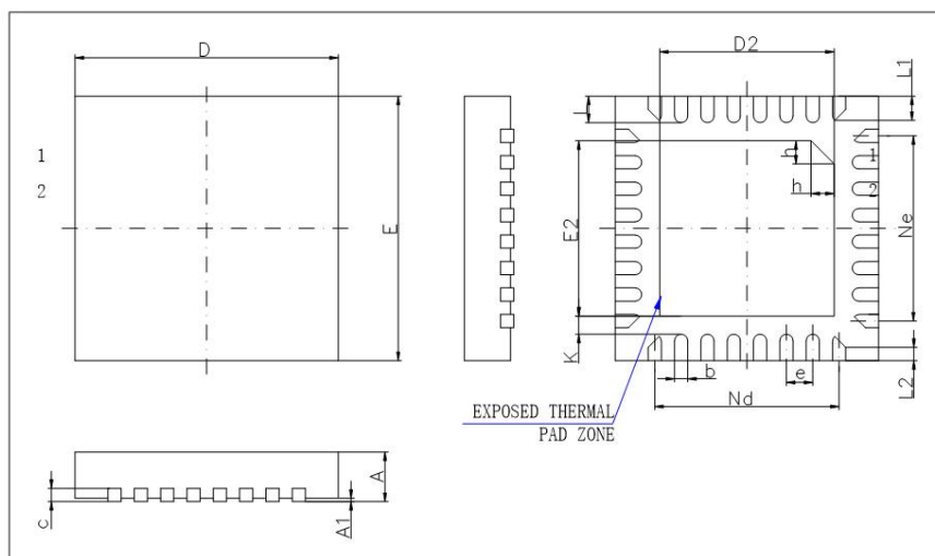
Figure 4-1 JL7106F Package
